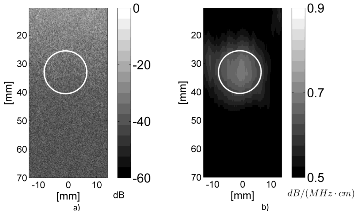
Fig. 7. The standard B mode image (a) and the attenuation map (b) present the attenuating object in tissue mimicking phantom. The attenuation of background and the object was equal 0.5 and 0.7 dB/(MHz·cm) respectively.
