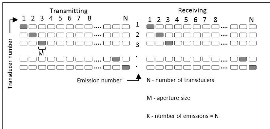
Fig.3 Scheme of SAF mode.
