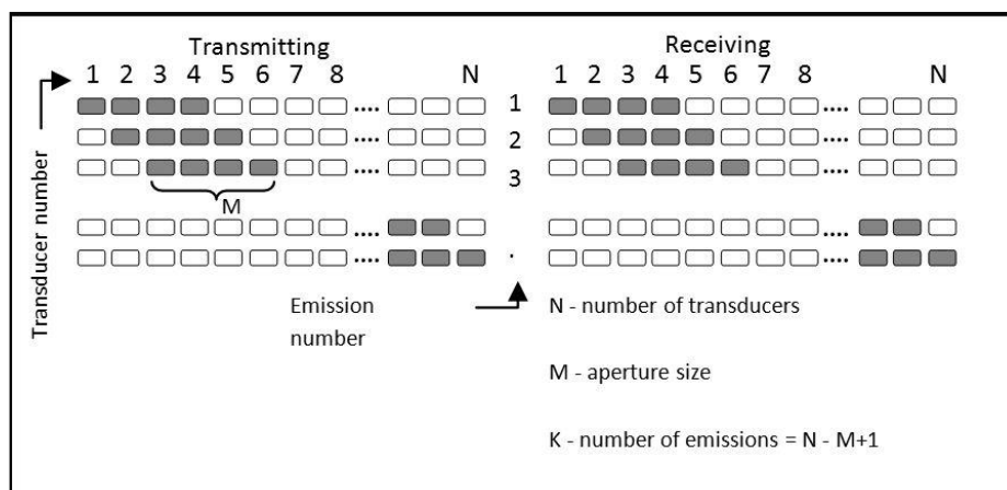
Fig.4 Scheme of M-SAF mode.
