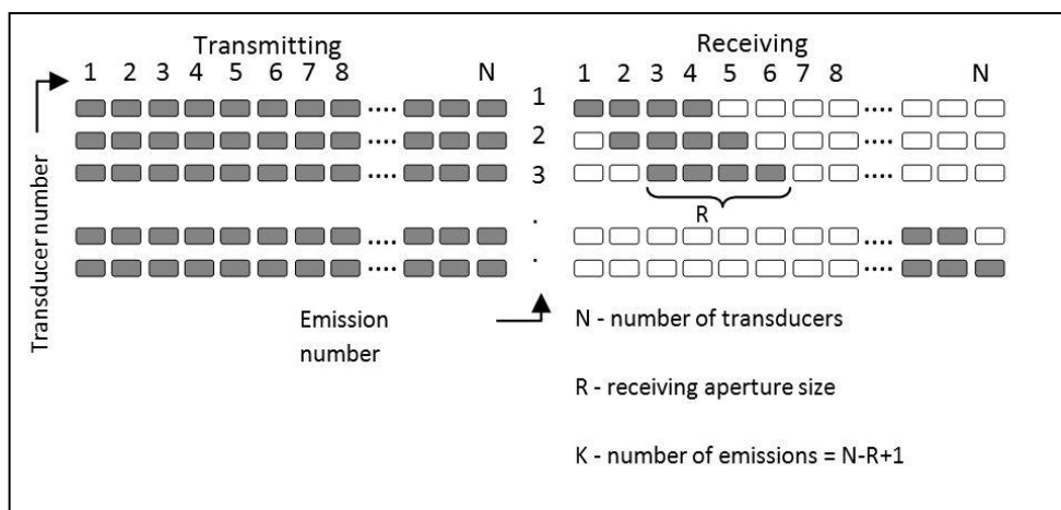
Fig.6 Scheme of SRA mode.
